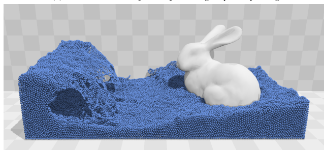
(b) Underlying simulation particles
