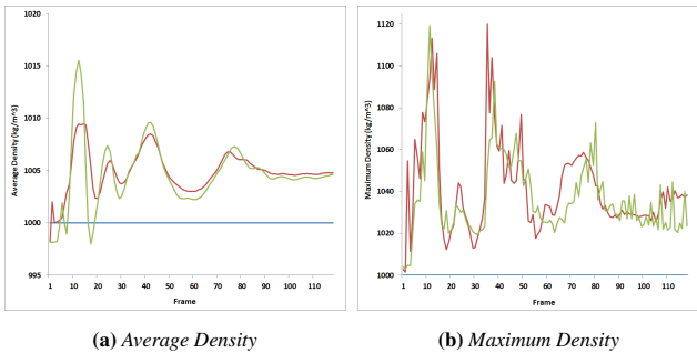
Figure 4: Density over the bunny drop simulation. Our algorithm maintains compressibility similar to PCISPH at time-steps more than twice as large. Color key: Blue, rest density. Red, PCISPH. Green, our method.
