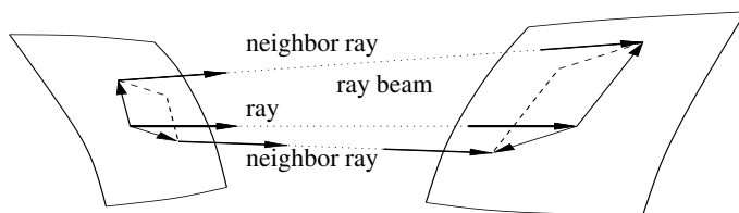
Figure 2.22: Rays and ray beam.
