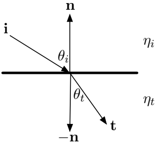
Figure 2.13: Refraction direction geometry.
