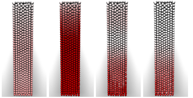
Fig. 4. Subsequent frames of a resting fluid pillar of 5 meters height, simulated at low resolution. The convergence criterion is set to a maximum density error of 1%. This leads to oscillations in the pressure field and, thus, the free surface. Pressure values are color coded, where red is maximum.
