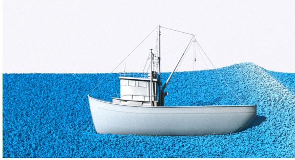
Figure 4: A two-way coupled boat, plausibly floating on 40M FLIP particles. The particles are not penetrating the solid object.
