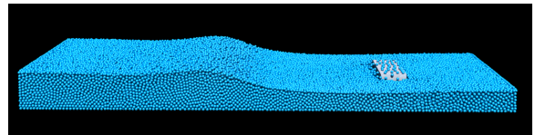
low-resolution IISPH ( h = 1.85\text{cm} )
