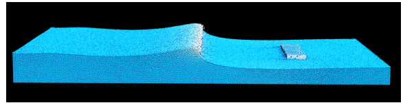
high-resolution IISPH ( h = 0.925\text{cm} )
