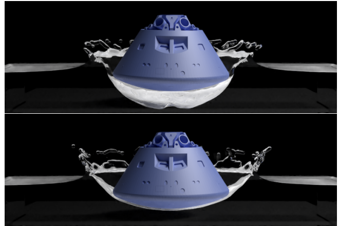
Fig. 4. Cutaway view of the Orion splashdown scene. The top image with a void region below the capsule is simulated using the method of Akinci et al. [2012]. The bottom image without void region is simulated with our two-way coupling approach.
