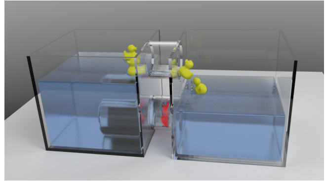
Fig. 3. A force-driven propeller pumps fluid from the right container to the left one using our approach. The time step is 3 ms, while [Akinci et al. 2012] requires a time step of 0.3 ms to obtain a stable simulation result.
