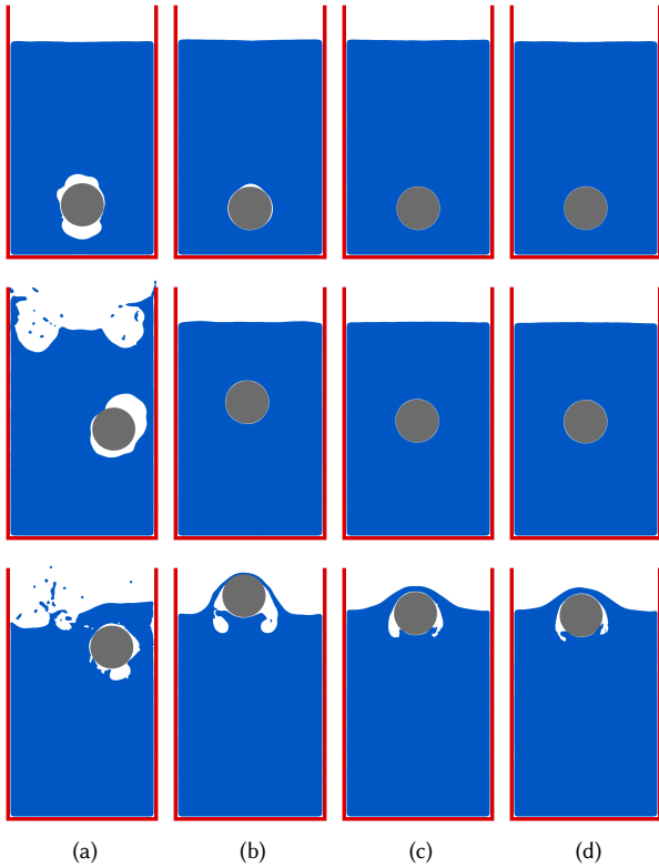
Fig. 2. 2D simulation of a rising sphere. (a), (b) and (c) show the method of Akinci et al. [2012] with time steps of 2 ms, 0.2 ms and 0.02 ms, respectively. (d) shows our approach with a time step of 2 ms.
